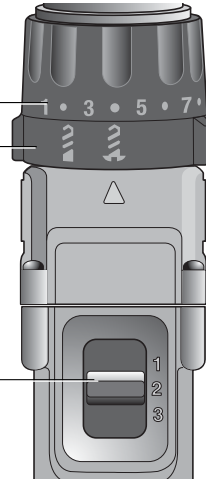
SCREWDRIVING
